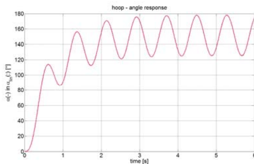
Fig.5 Hoop - angle response
