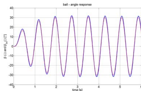
Fig.5 Ball - angle response
