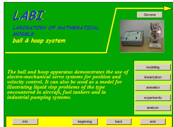
Fig.3 Ball & hoop system (TQ CE9) presentation
